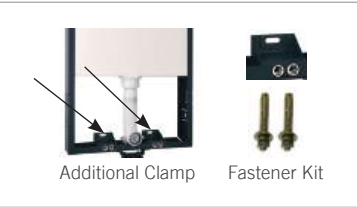
Unmatched Strength Metal Frame with additional clamps and fastener kit provide sufficient strength to withstand load of 400kg
